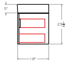
SIDE SECTION
